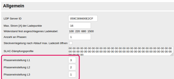
(Abb. 7: Phasenmapping)
